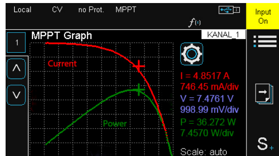
U/I and U/P characteristic curve on the user interface
