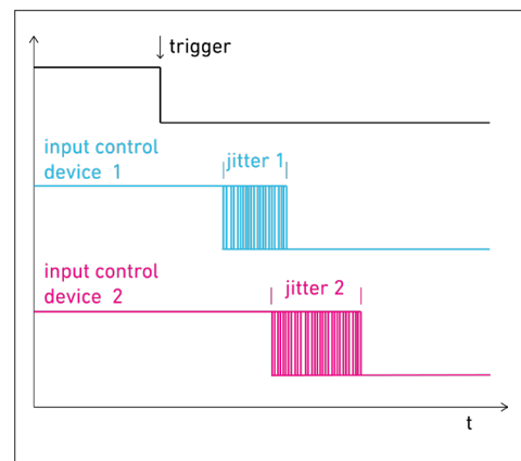
Jitter when repeatedly switching the load input on different series devices
