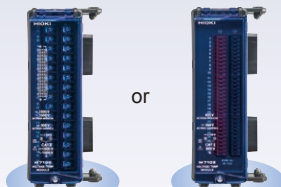
M7100 15 channels (voltage, temperature) M7102 30 channels (voltage, temperature)
