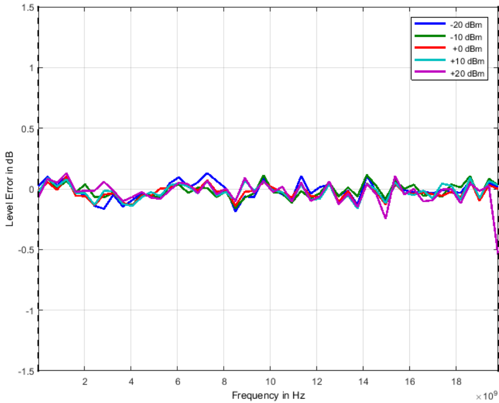
Typical Output Power Linearity (APULN20)
