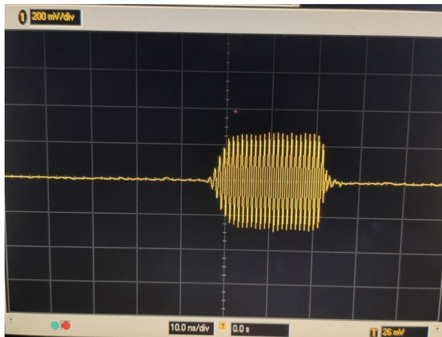
Internal Pulse Modulation (1 GHz, 20 ns pulse width)
