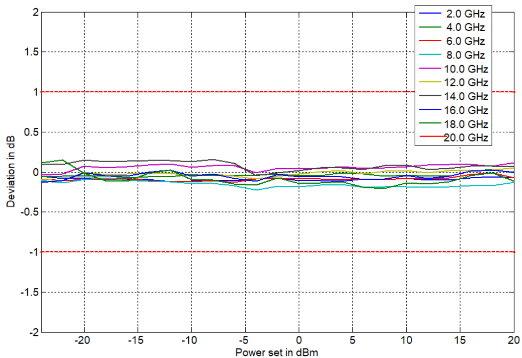
Typical Output Power Linearity (APULN20)
