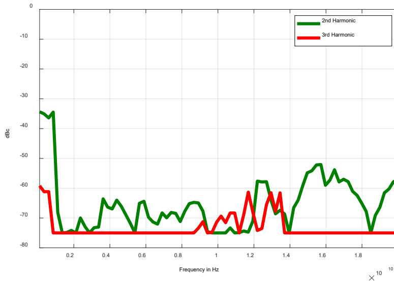
Harmonics (2nd, 3rd at P=+5 dBm, APULN40 with option FILT)
