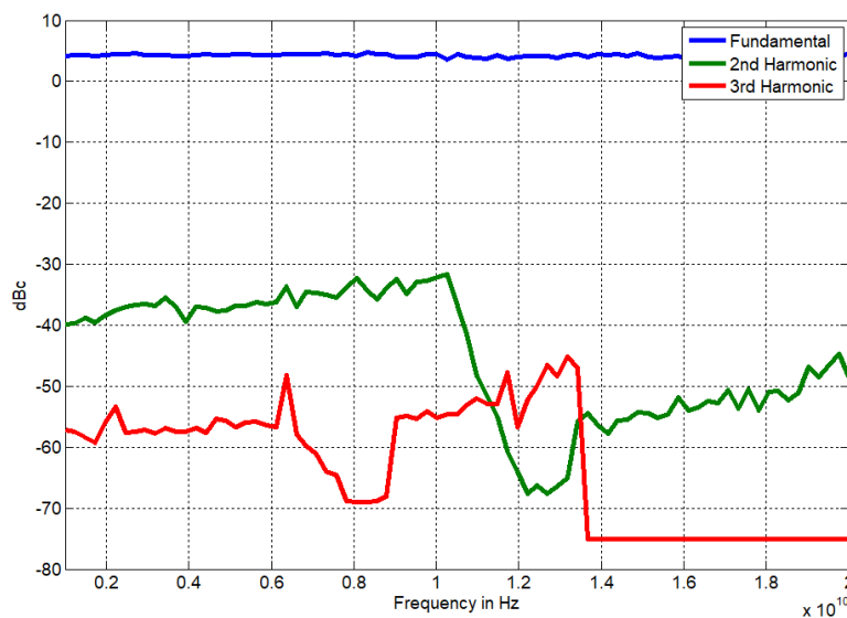
Harmonics (2nd, 3rd at P=5 dBm, APULN20)
