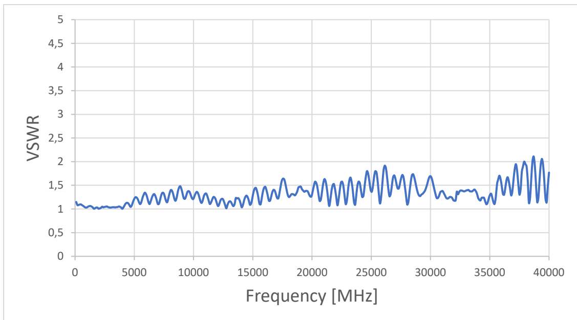
Figure 10: VSWR
