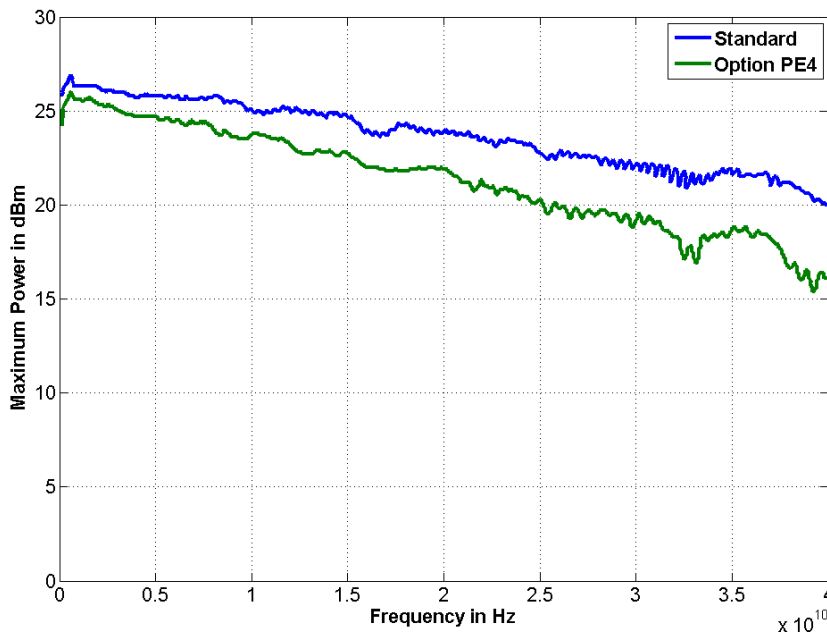
Figure 5: Maximum Output Power APMS40G with and without Option PE4
