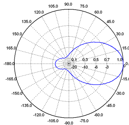
H-Ebene / H-Plane 200 MHz
