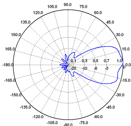
E-Ebene / E-Plane 1000 MHz
