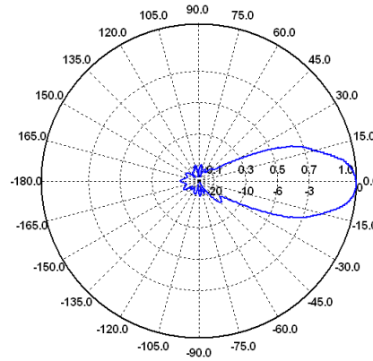
H-Ebene / H-Plane 1.2 GHz
