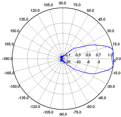
E-Ebene / E-Plane 1.8 GHz
