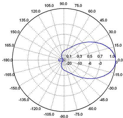
E-Ebene / E-Plane 300 MHz
