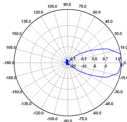
H-Ebene / H-Plane 1.6 GHz
