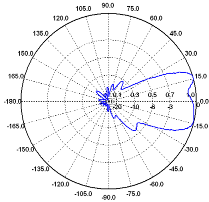
E-Ebene / E-Plane 1.2 GHz
