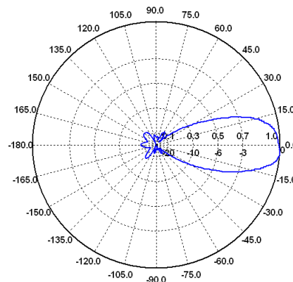
H-Ebene / H-Plane 1000 MHz
