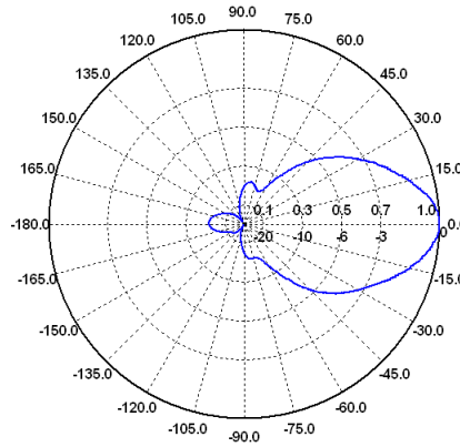
H-Ebene / H-Plane 500 MHz
