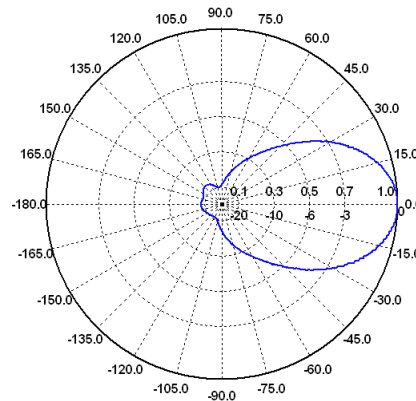
H-Ebene / H-Plane 300 MHz
