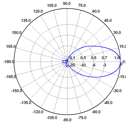
H-Ebene / H-Plane 400 MHz
