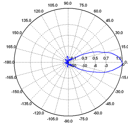
H-Ebene / H-Plane 1.8 GHz
