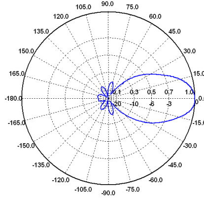
H-Ebene / H-Plane 600 MHz
