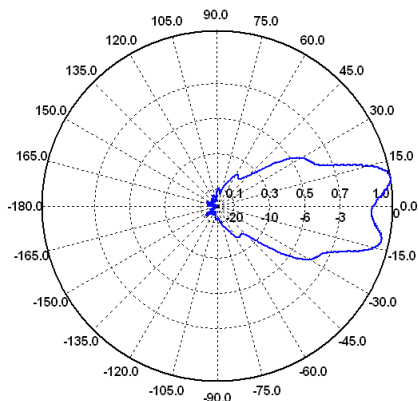
E-Ebene / E-Plane 1.6 GHz
