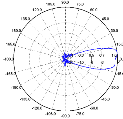
H-Ebene / H-Plane 2 GHz
