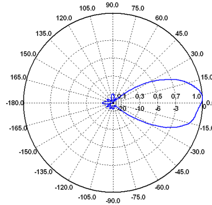
H-Ebene / H-Plane 900 MHz
