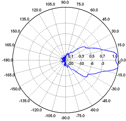
E-Ebene / E-Plane 2 GHz
