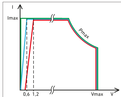
Operating range of different DC loads
