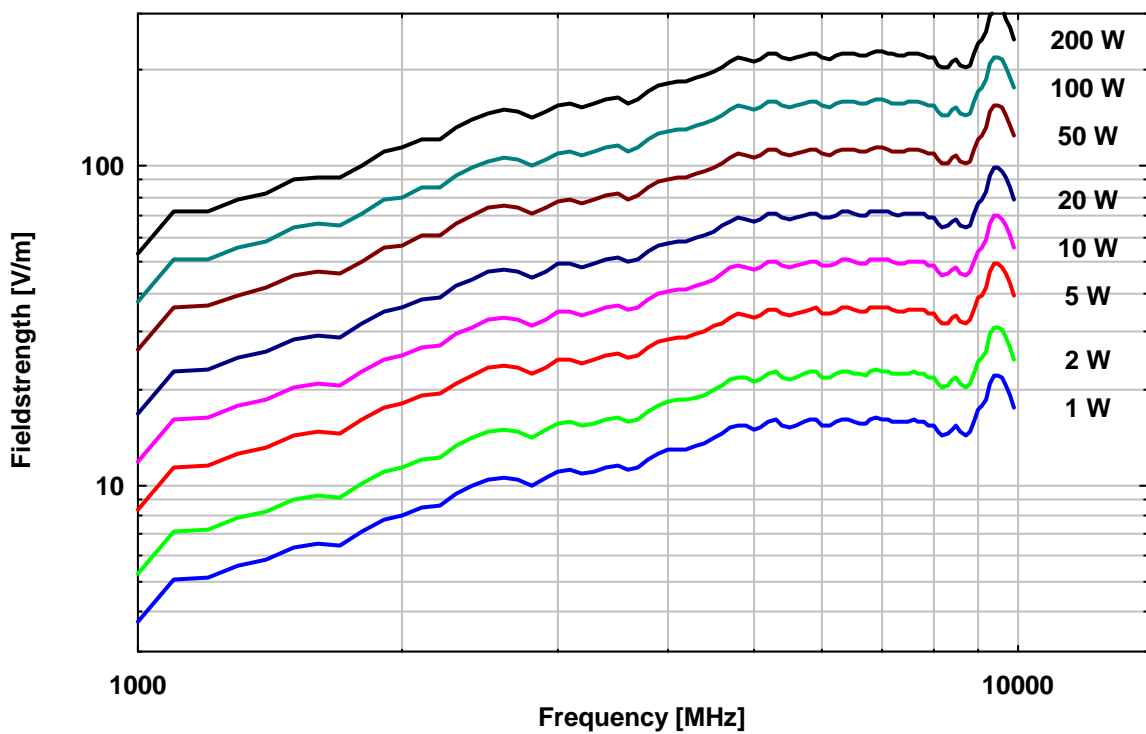
BBHA 9120 B Input Power, Dist. Aperture-EuT: 2 m
