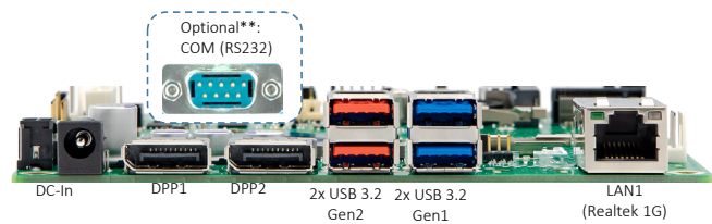
*) Prepared for SMARTCASE™ S501 chassis kit **) Via optional COM port cable. Breakout feature 5C501 chassis rear I/O
